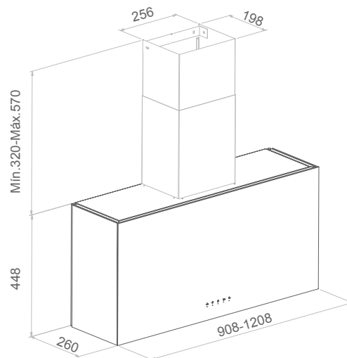
Dimensions in mm Special Custom-Made Flues Flue included as standard with the ducted version
