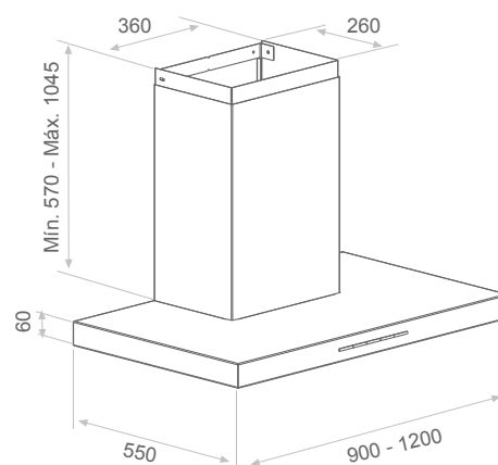
Dimensions in mm Special Made-to-Measure Flues
